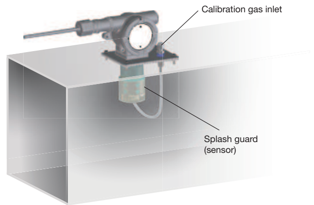
[Duct insertion type]
