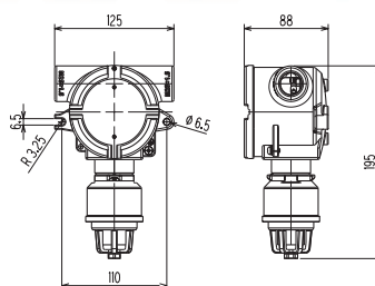
Remote sensor unit (GD-3 Series) Diffusion type without EC barrier
